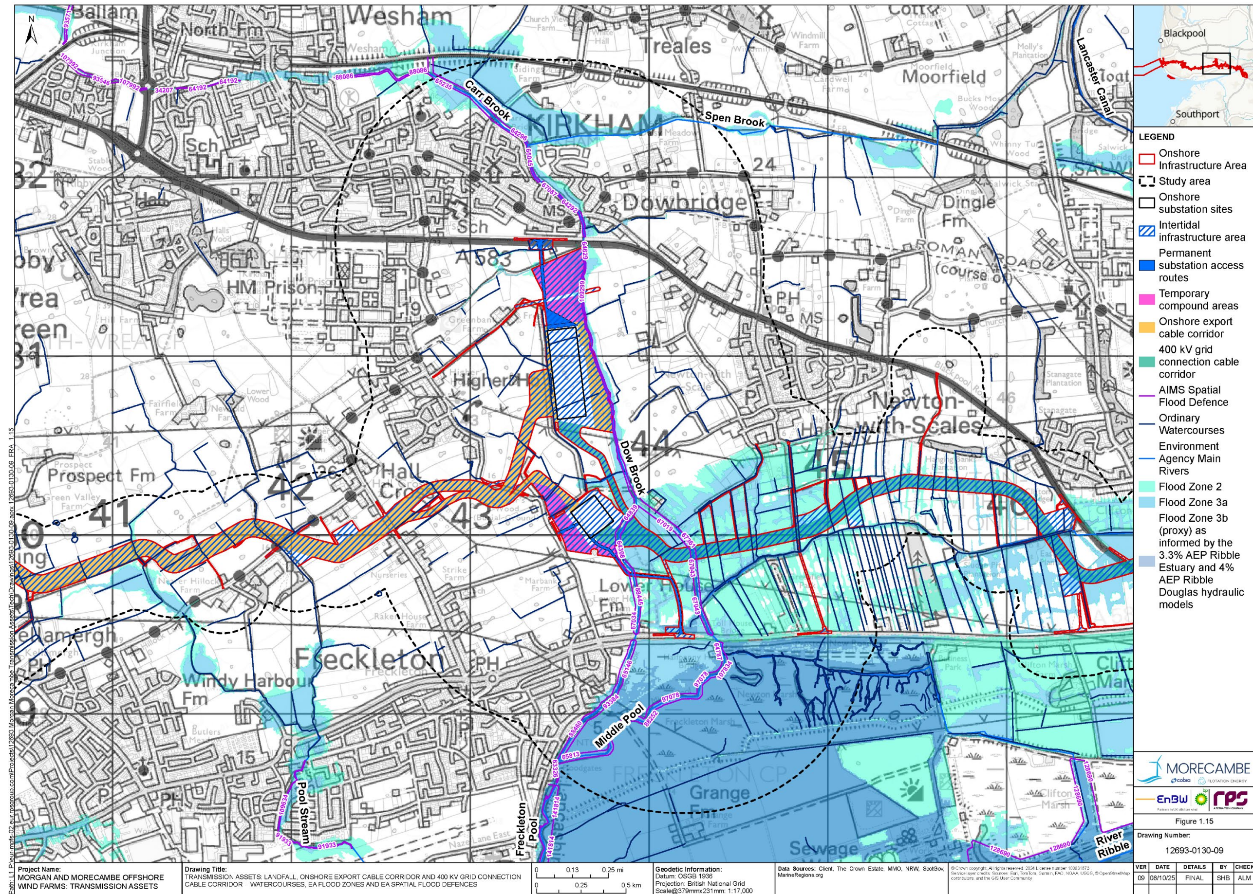
Figure 1.15: Transmission Assets: landfall, onshore export cable corridor and 400 kV grid connection cable corridor - Watercourses, EA Flood Zones and EA Spatial Flood
