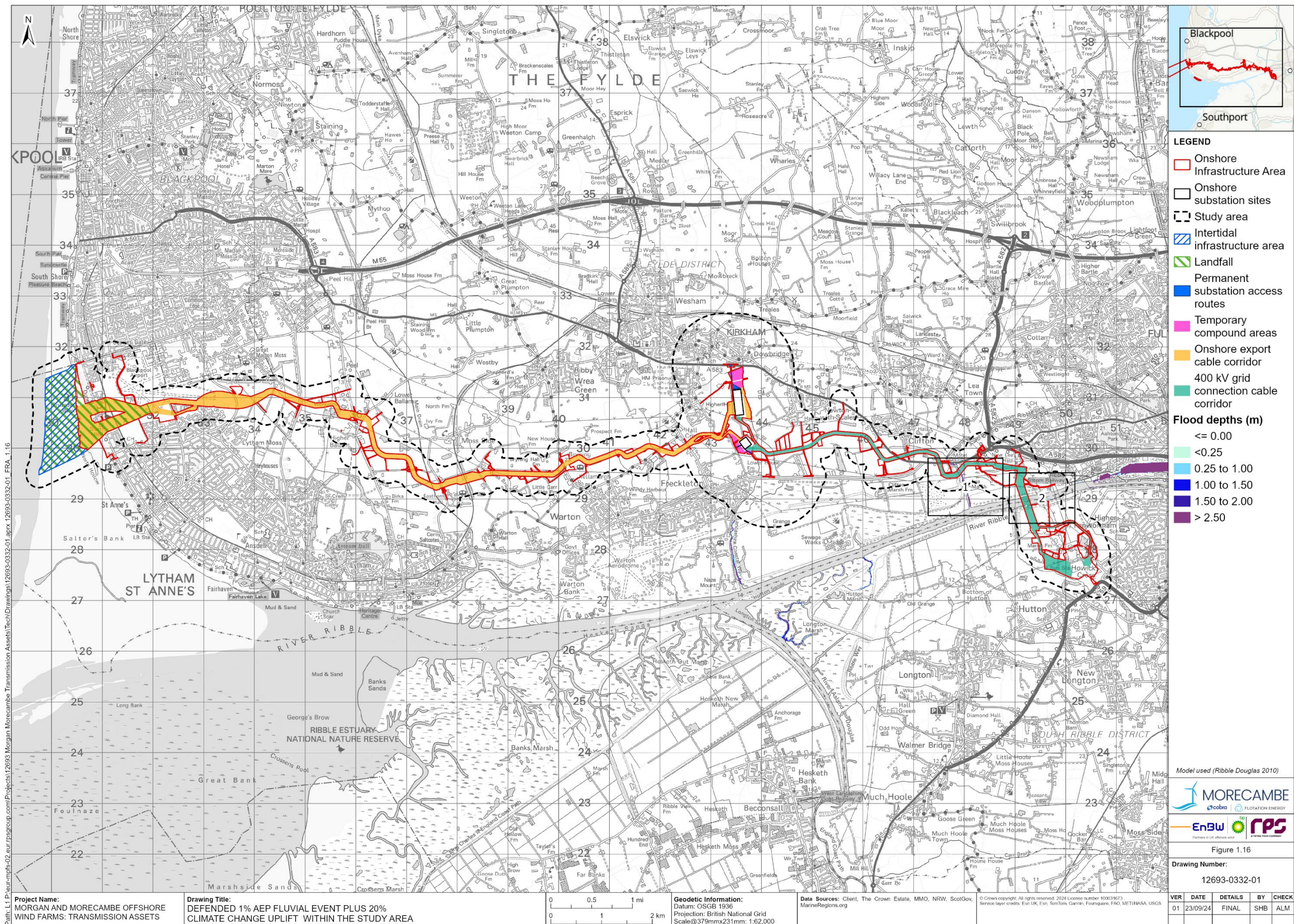
Figure 1.16a: Defended 1% AEP fluvial event plus 20% climate change uplift within the study area
